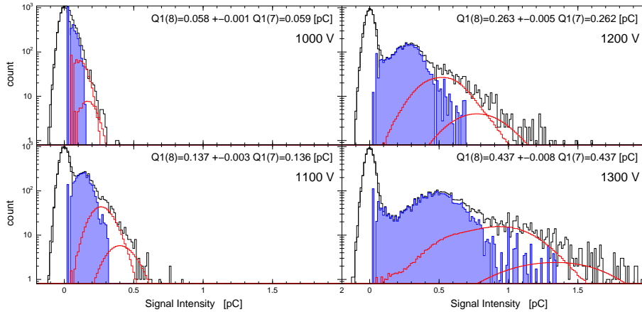
Fig. 6. Estimates of 1 PESD obtained with various PMT gains. The average signal from single photoelectrons \langle Q_1 \rangle , as estimated from Equations 7 and 8, are also indicated in each panel. The statistical error is inversely proportional to the square of the number of events, which is 10,000 in the measurements shown in this figure.
