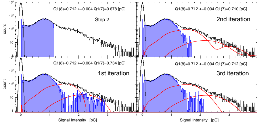
Fig. 3. Distribution of signal from the PMT. A high voltage (1400 V) was applied to the PMT and the signal was amplified by a preamplifier with a gain of 24. We measured 100,000 events with the shutter open. The signal from these events is shown by the black-line histogram. We also determined the quantity 0 PESD, or n_0(i) , by measuring 100,000 events with the shutter closed; this is also shown by a black-line histogram. The quantity 1 PESD, or n_1(i) , is shown by the shadowed histogram, and the distributions corresponding to 2 and 3 PESDs are shown by (red) solid lines. Our initial estimate of 1 PESD, obtained in Step 2 (see text), is shown in the upper left panel. The result of the first iteration in Step 4 is shown in the lower left panel, and the second and third iterations are shown in the right panels. Four iterations proved sufficient to converge the PESDs. The average signal corresponding to a single photoelectron, as obtained from Equations 7 and 8, are also indicated in each panel.
